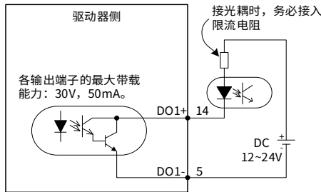
②接光耦
